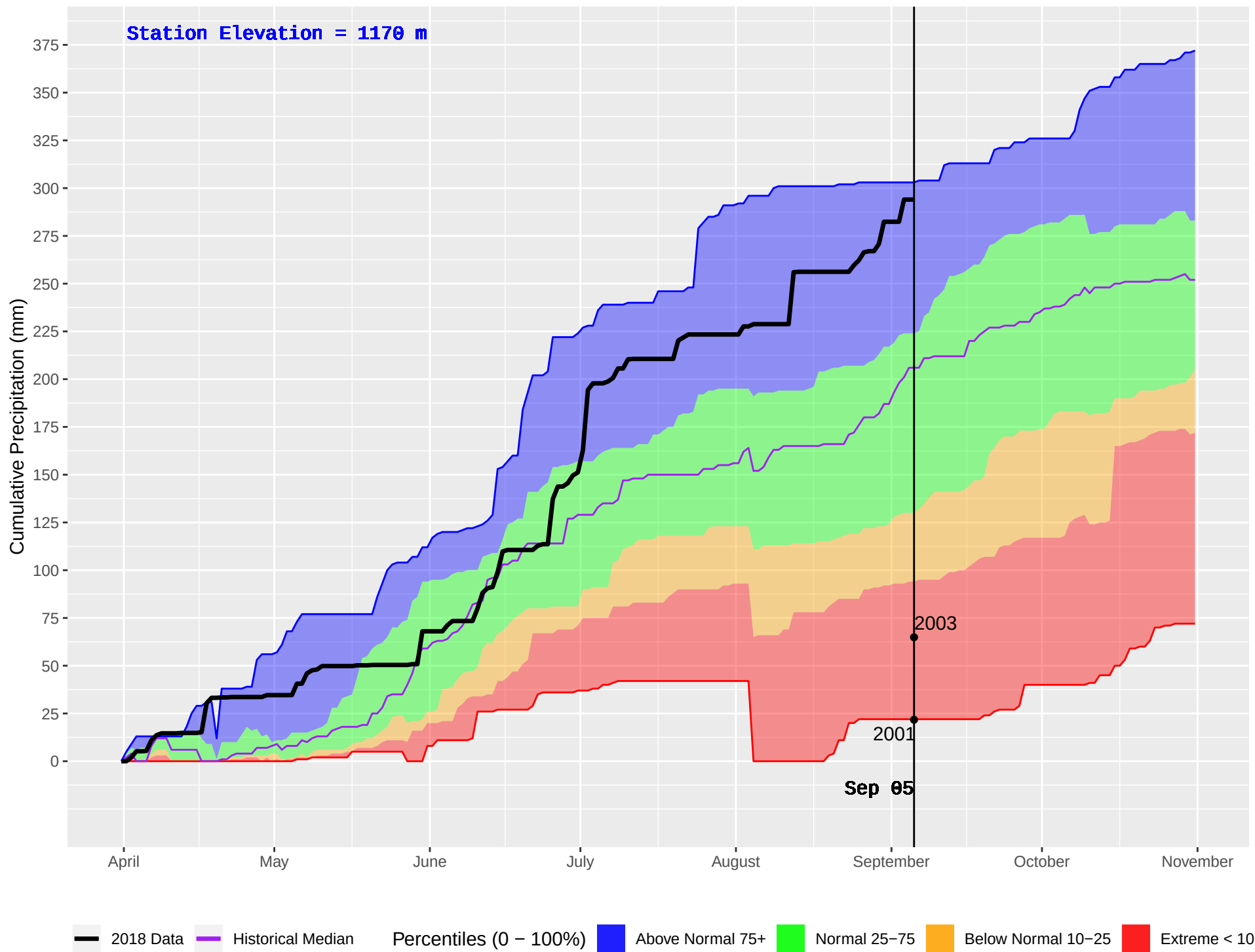
YOUNG LAKE (235) : Historical (2001–2016) and Current (2018) Daily Cumulative Precipitation
