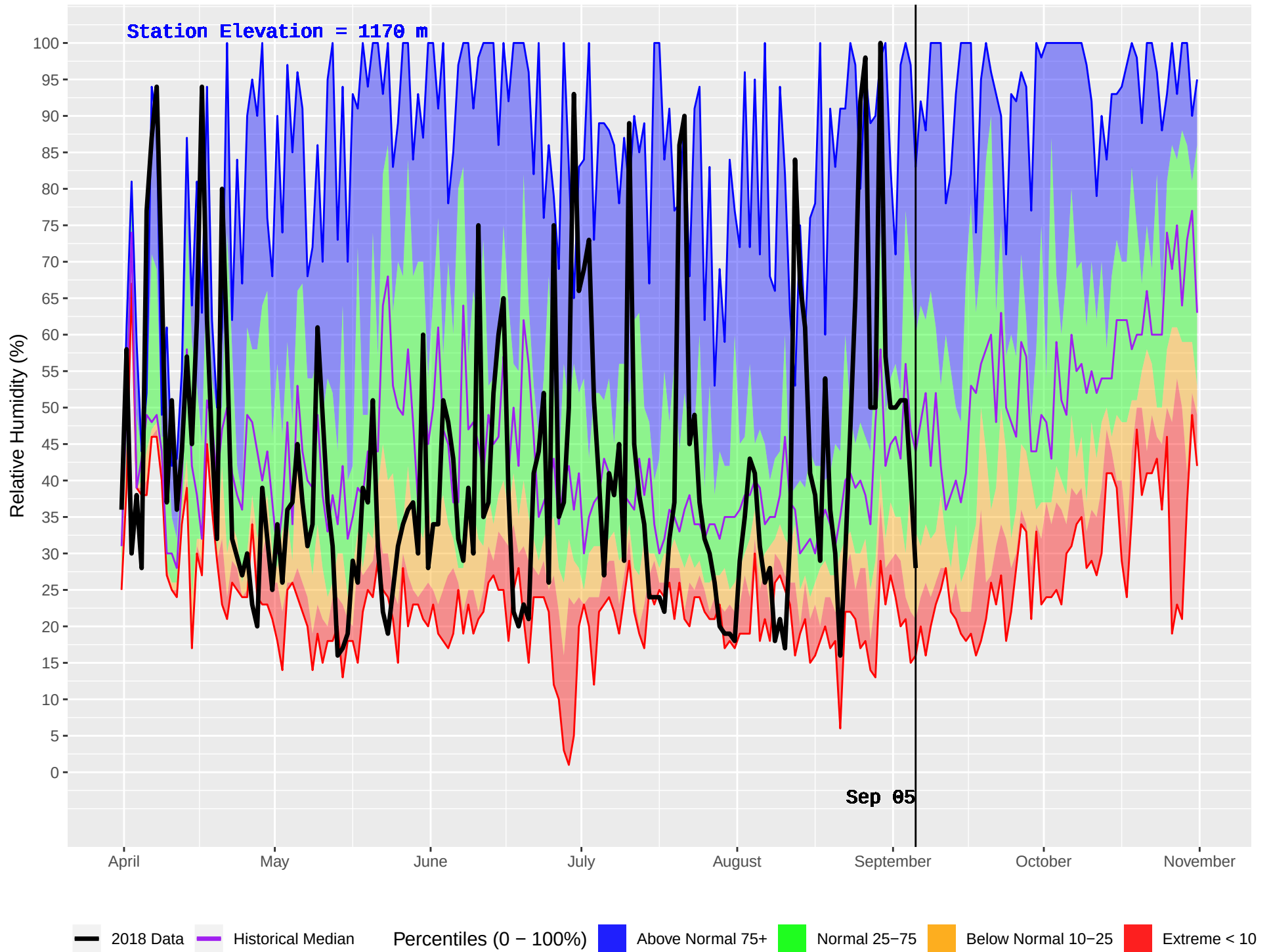
YOUNG LAKE (235) : Historical (2001–2016) and Current (2018) Daily Relative Humidity
