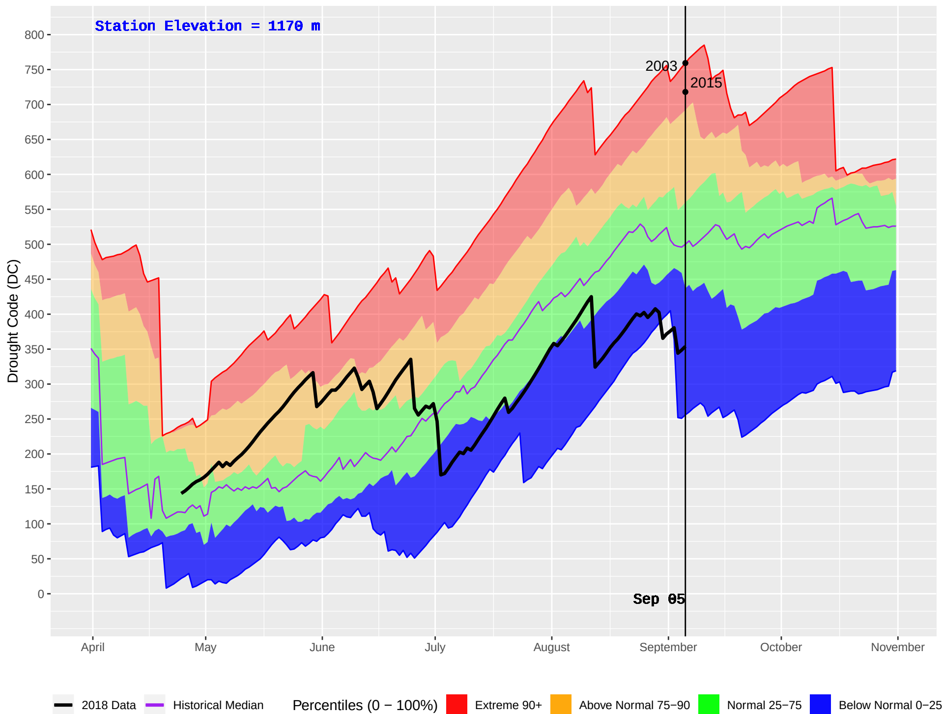
YOUNG LAKE (235) : Historical (2001–2016) and Current (2018) Daily Drought Code (DC)
