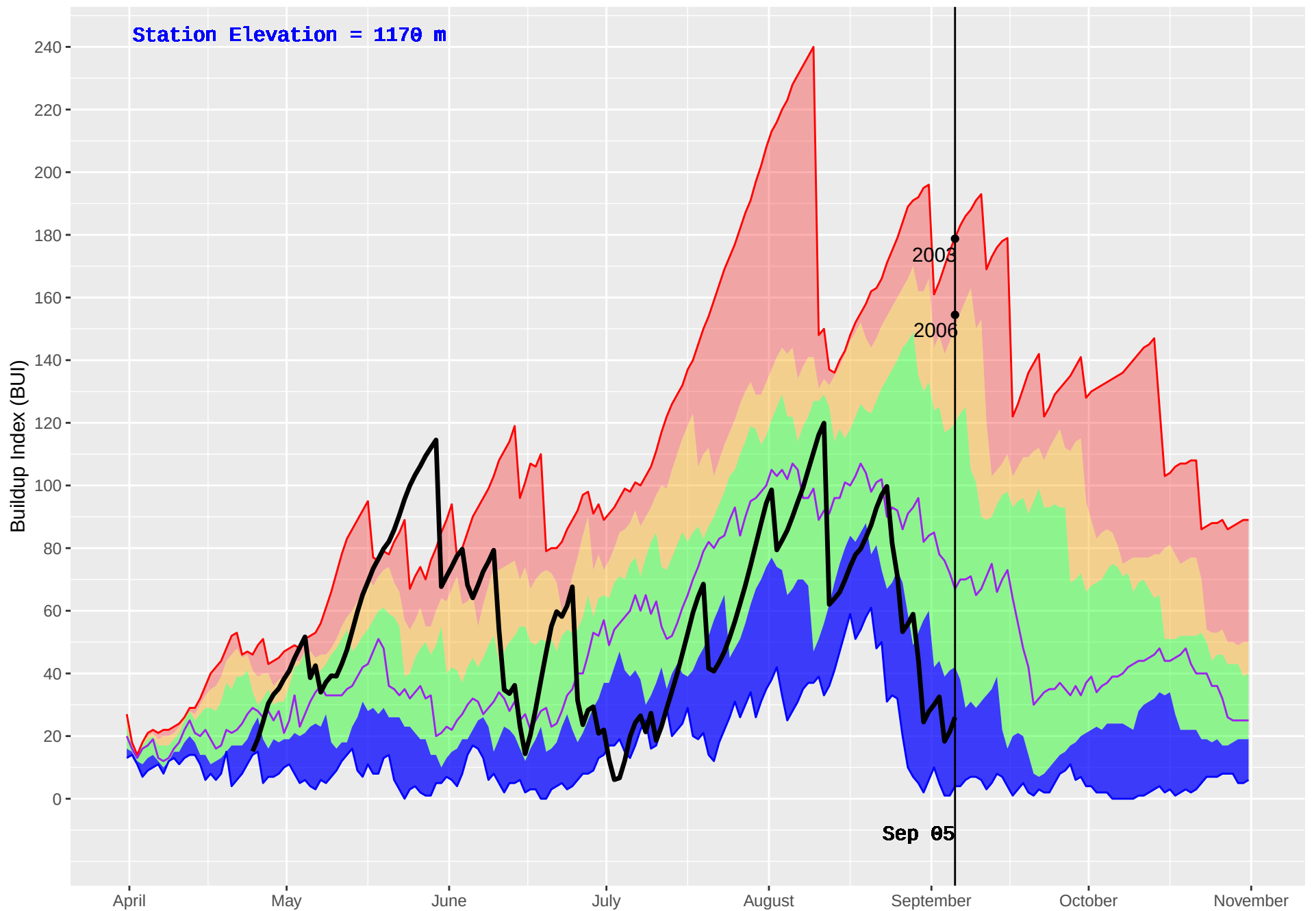
YOUNG LAKE (235) : Historical (2001–2016) and Current (2018) Daily Buildup Index (BUI)
